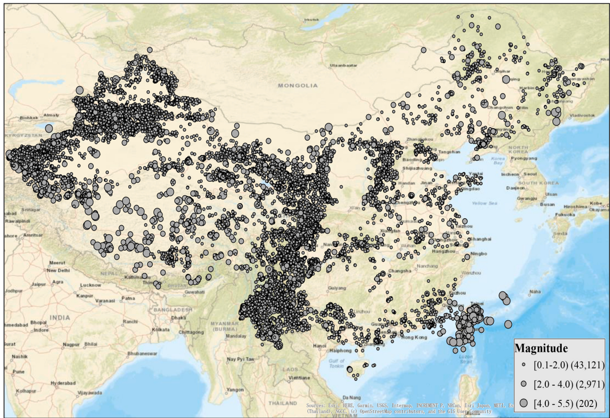
Fig. A2. Distribution of the earthquakes recorded across China in 2009.
