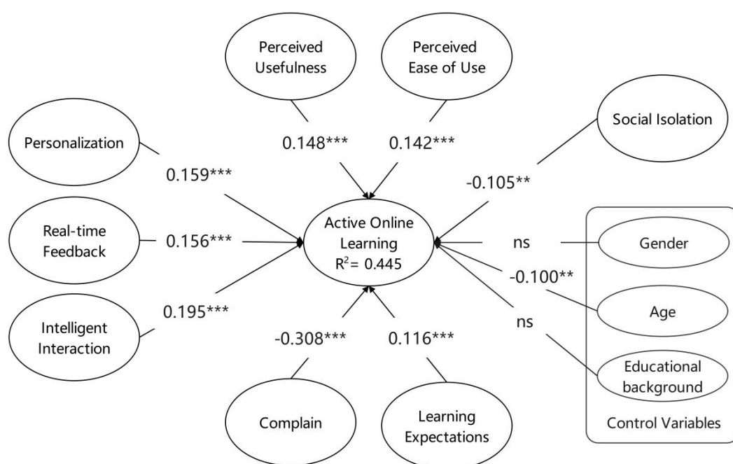
Figure 2. Structural model PLS results.
